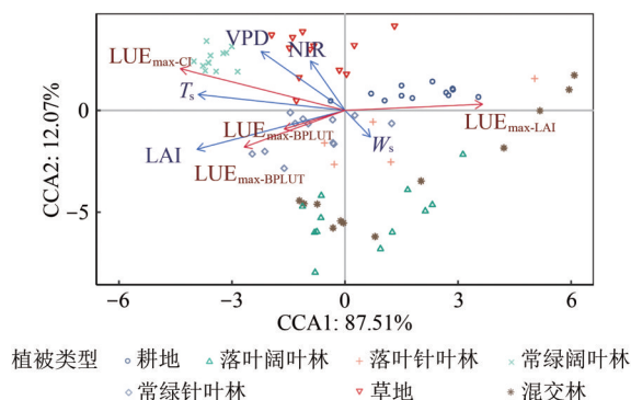
图5 LUE_{\max} 参数与环境影响因素间的相关性分析 Fig. 5 Correlation analysis between LUE_{\max} parameters and environmental influencing factors
